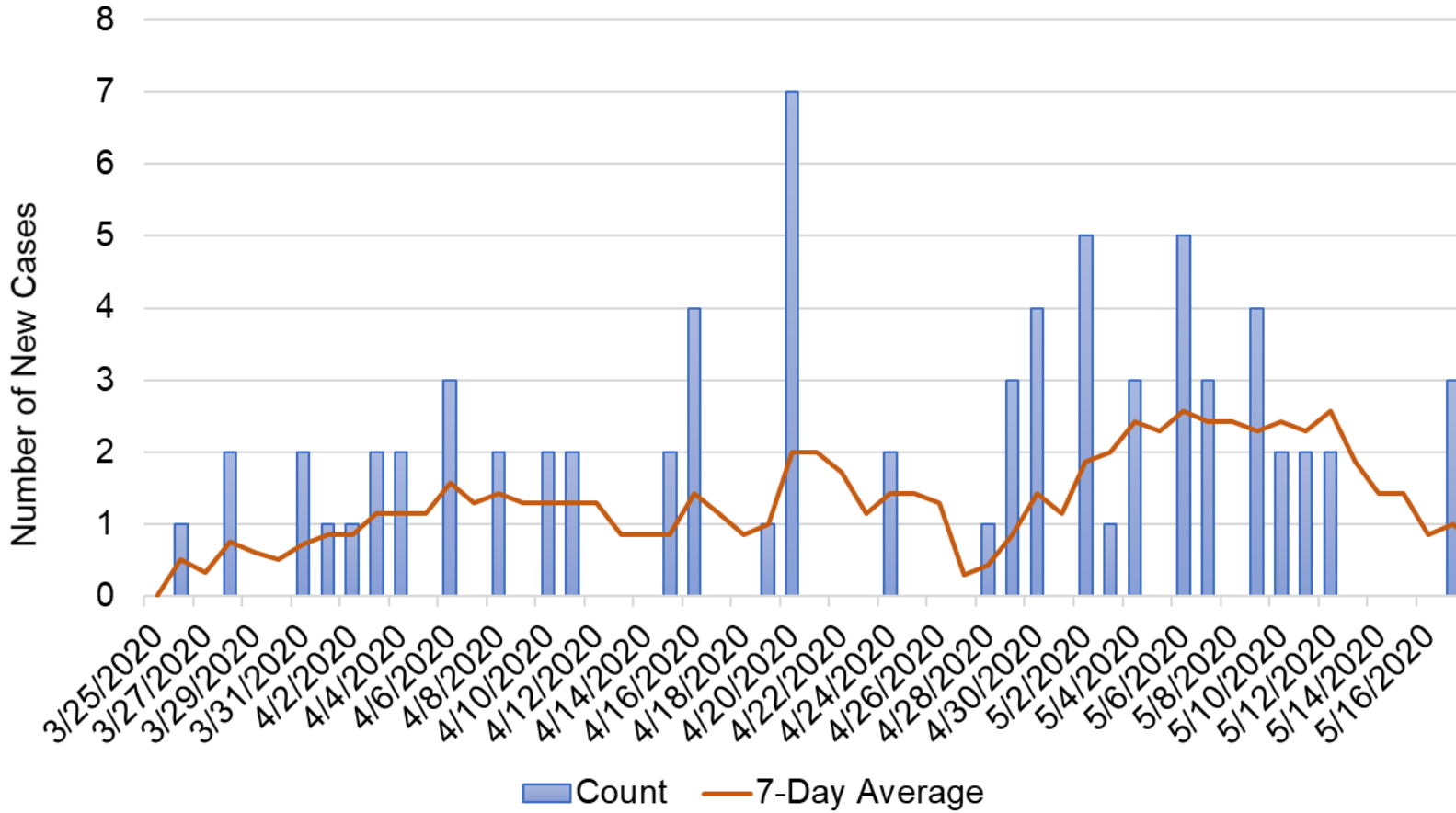
New Cases by Day and Seven-Day Average
